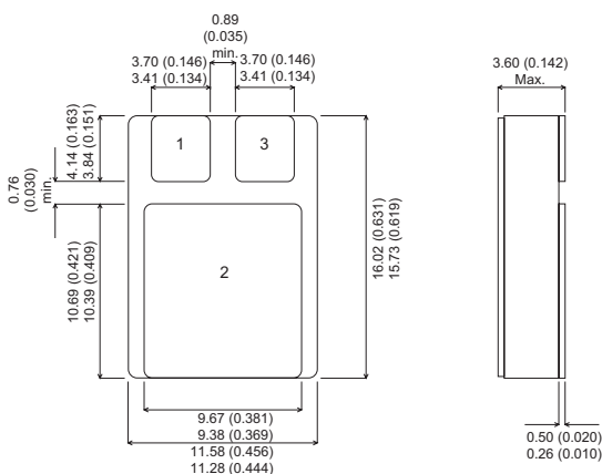
SMD1 (TO-276AB)
